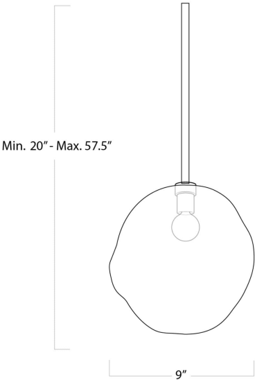
Canopy: 5" Dia. x .75"
