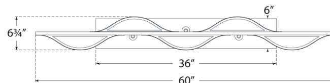
Bottom View
